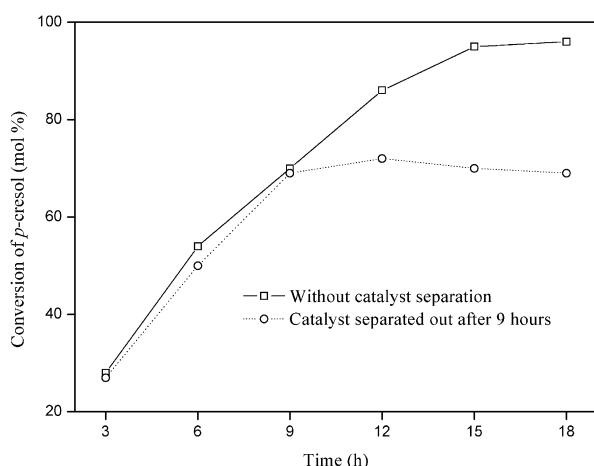
Figure 6. Influence of catalyst separation. Reaction conditions: catalyst (CuMn/carbon, Cu:Mn=4:1)=0.6 g, p -cresol=16.0 g, solvent (methanol)=50 mL, sodium hydroxide=23.0 g, pressure=0.1 MPa, temperature=348 K, stirring speed=700 r.p.m.
